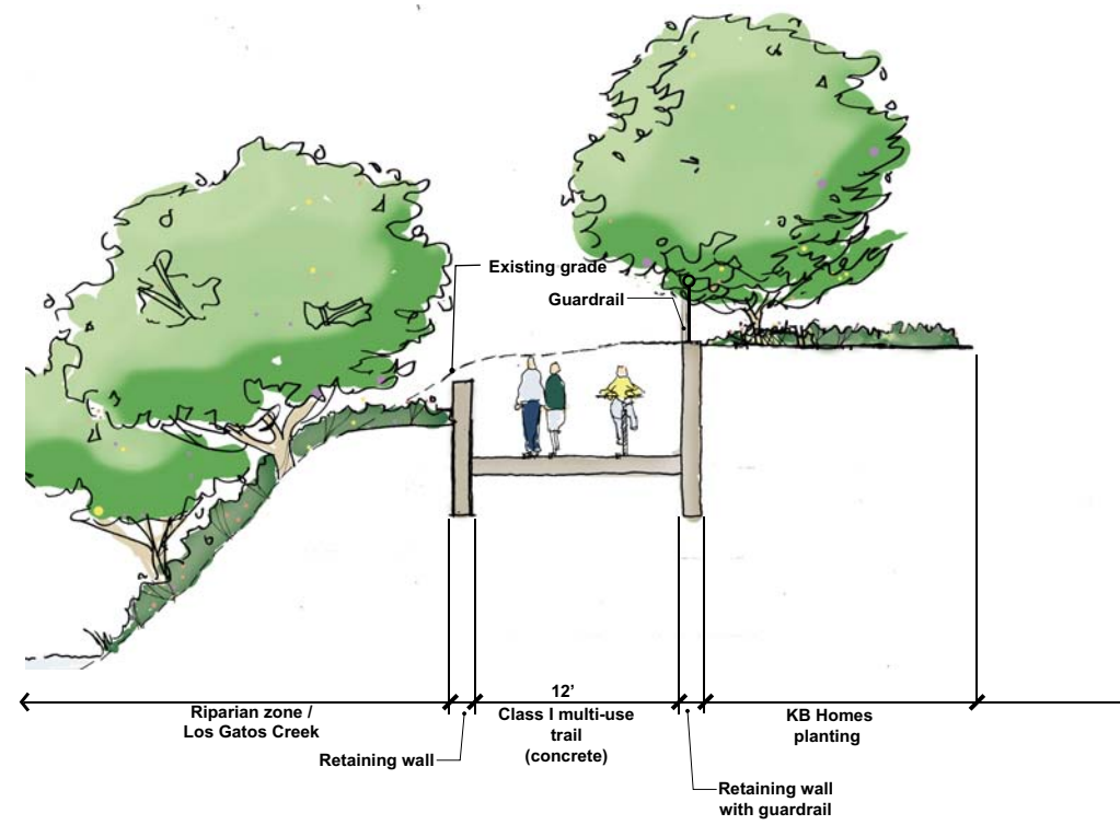
B Section West San Carlos St. Undercrossing
