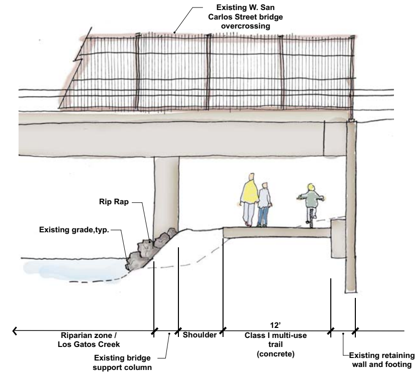
C Section West San Carlos St. Undercrossing
