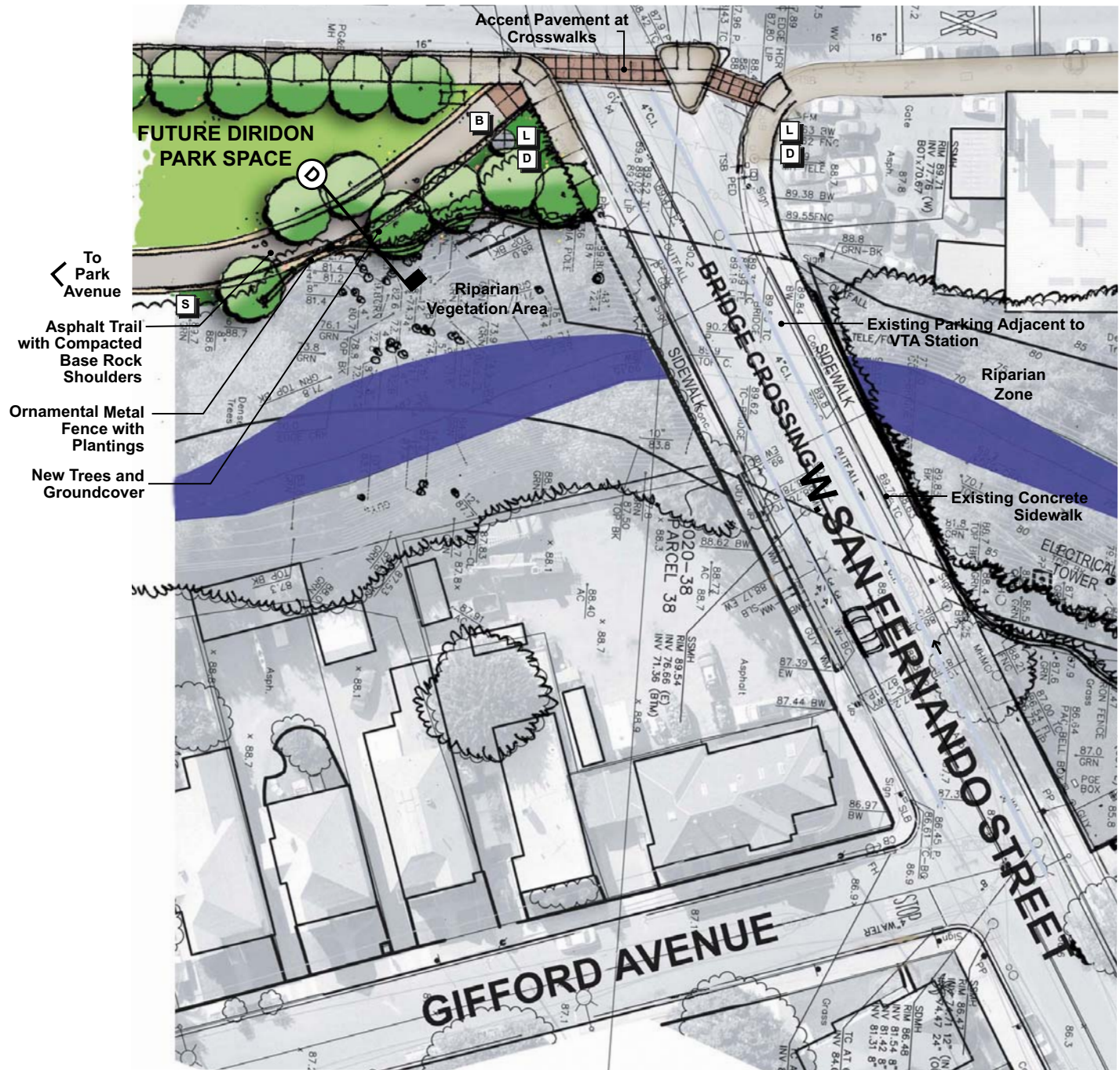
3 West San Fernando Street Enlargement Plan
